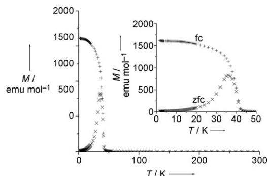
Figure 4. DC magnetization of \text{Mn}_3\text{O}_4 nanoparticles measured after cooling in zero field (zfc, \times ) then in a field of 0.01 T (fc, + ). The inset reveals the responses near the fc–zfc splitting in greater detail.
